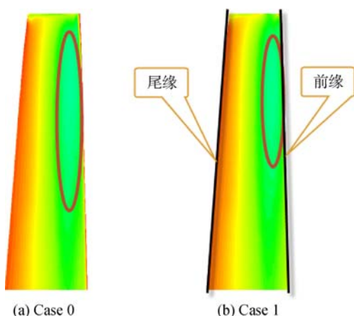
Fig. 11 Distribution of pressure on the pressure side of blade tip
